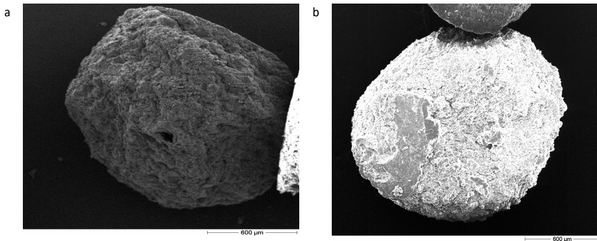
Fig. 2: SEM of Theophylline microbeads containing: a, pregelatinized breadfruit starch- alginate blend as polymer and b, sodium alginate alone
